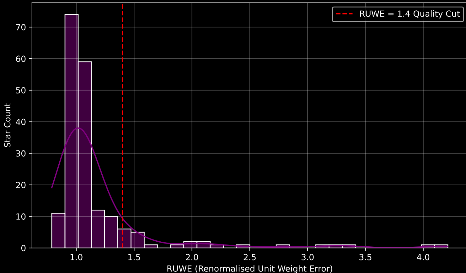
GAPOGEE DR17 Field [022+82_MGA] RUWE Distribution (n= 191)
