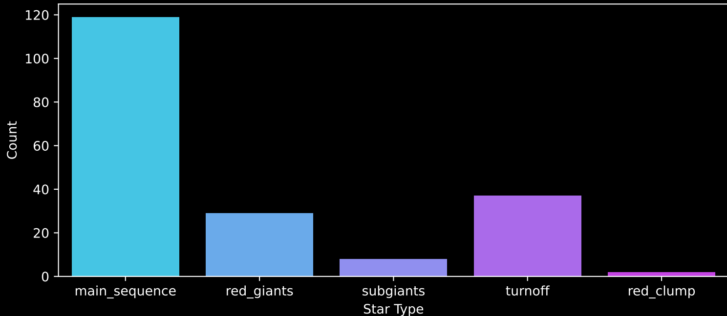
APOGEE DR17 Field: [022+82_MGA] Count plot of Star Type
