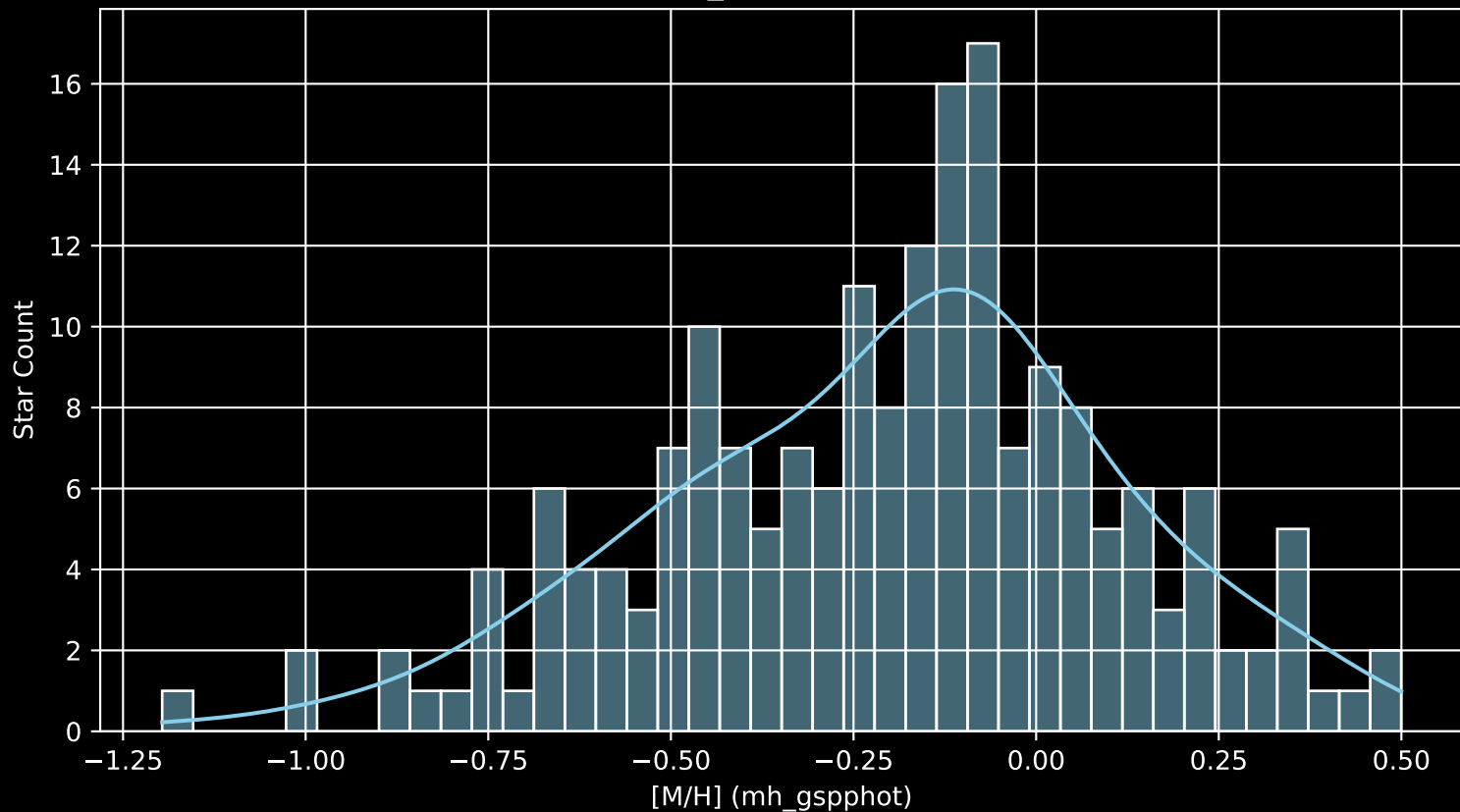
APOGEE DR17 Field: [022+82_MGA [M/H] (mh_gspphot) (n= 192)
