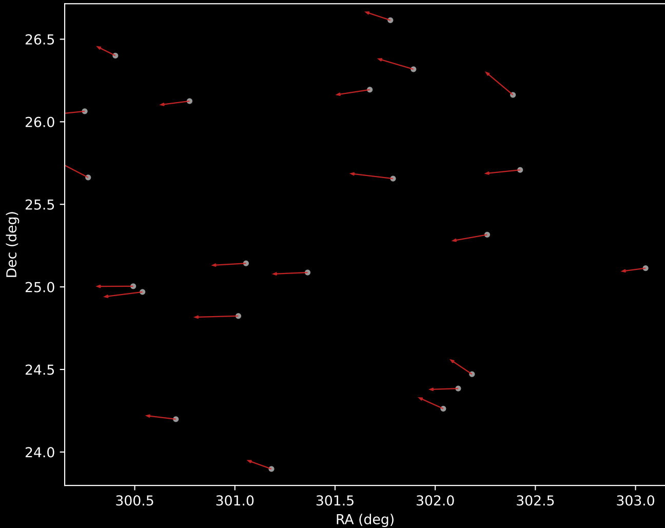
APOGEE DR17 Cluster 6 Proper Motion Vectors (n=22)
