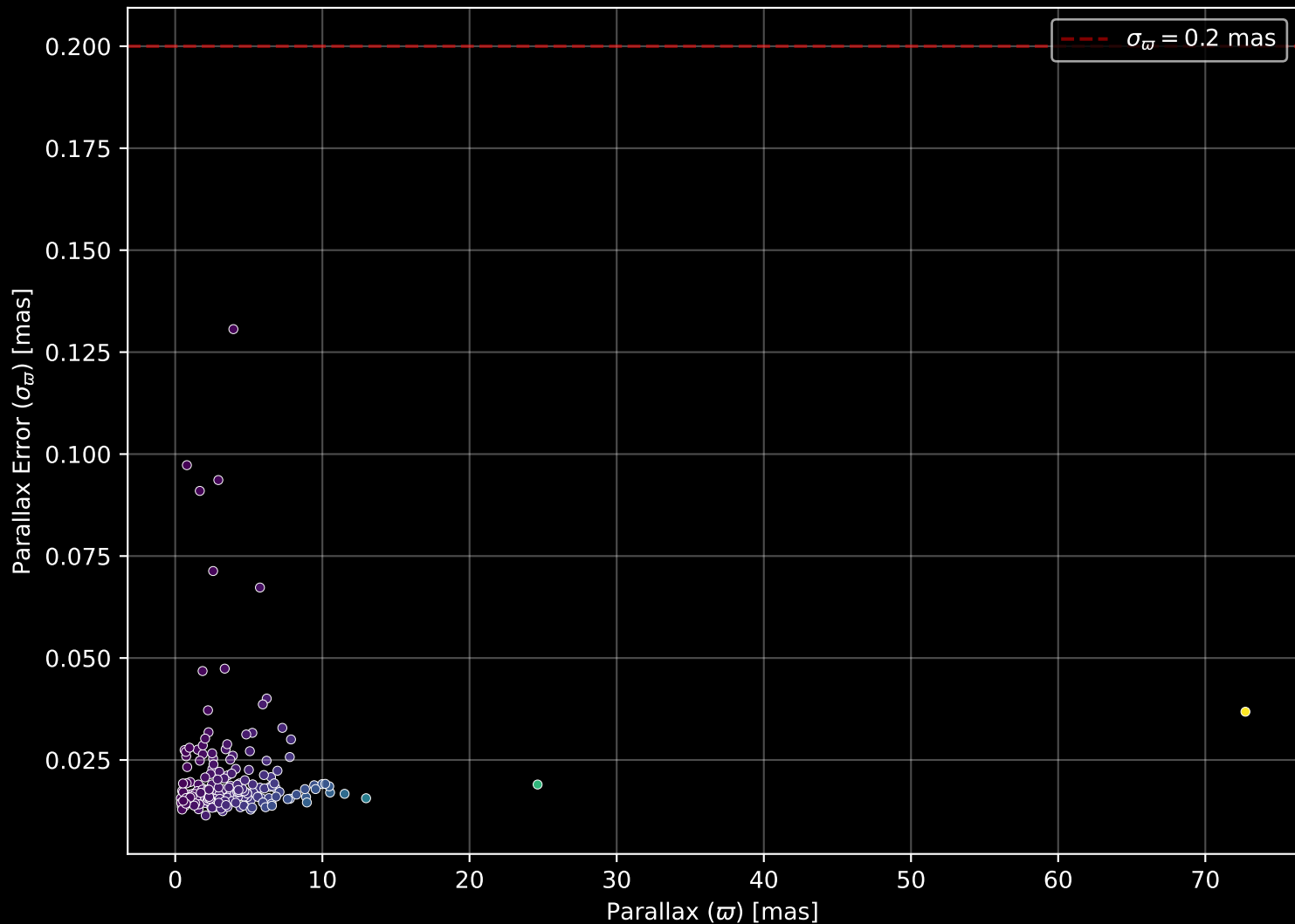
APOGEE DR17 Field: [022+82_MGA] Parallax Quality (n= 195)
