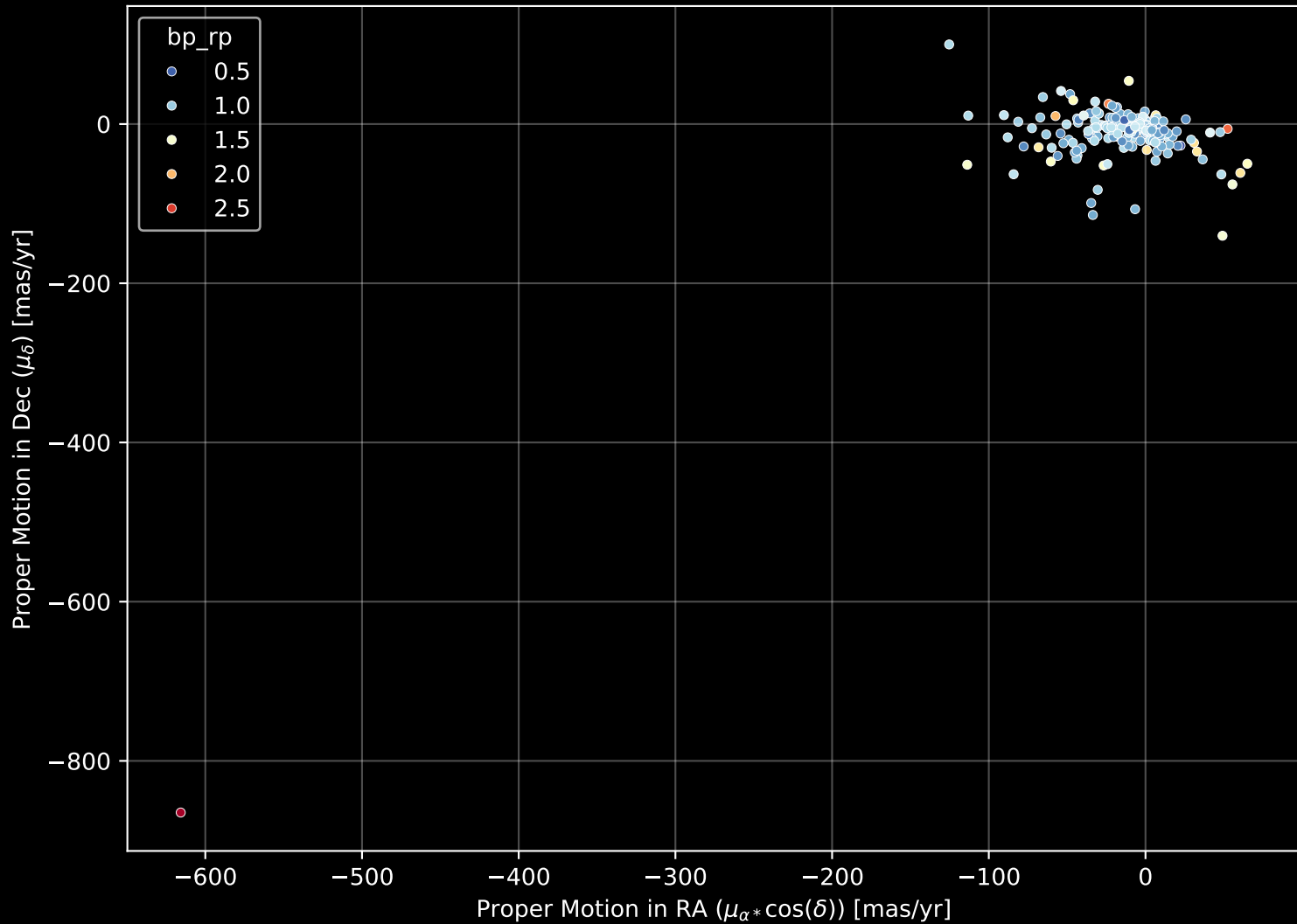
APOGEE DR17 Field: [022+82_MGA] Proper Motion Diagram (n= 195)
