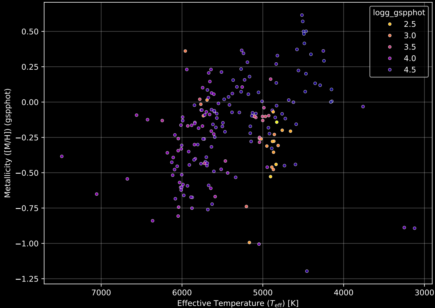
APOGEE DR17 Field: [022+82_MGA] Stellar Population Parameters (n= 195)
