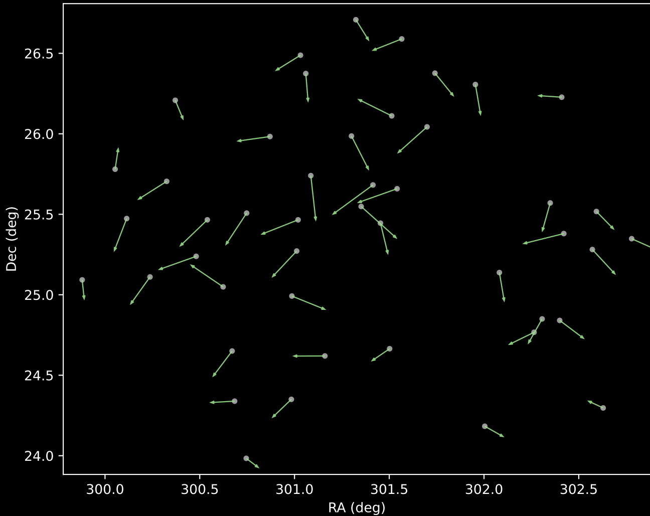
APOGEE DR17 Cluster 5 Proper Motion Vectors (n=46)
